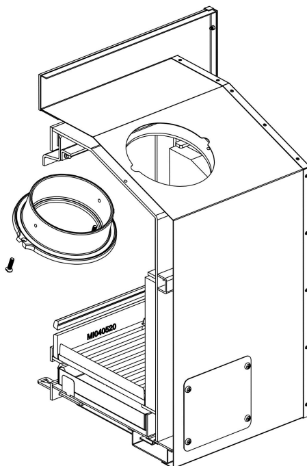
Figure 2.1 Section view of flue collar & fixing bolts.
