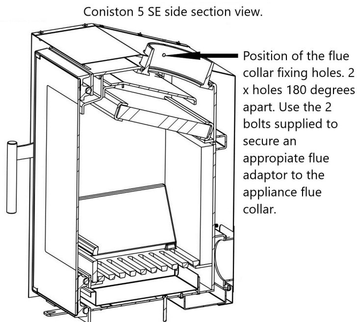
Figure 2.5 Flue collar holes for retaining a flue adaptor.
