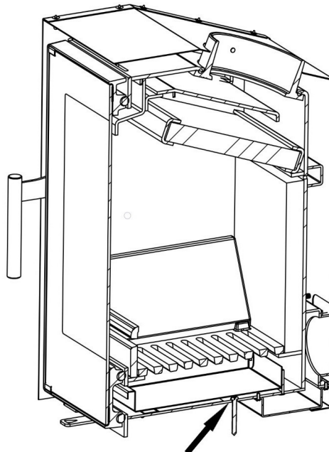
Figure 2.3 Appliance fixing position.
