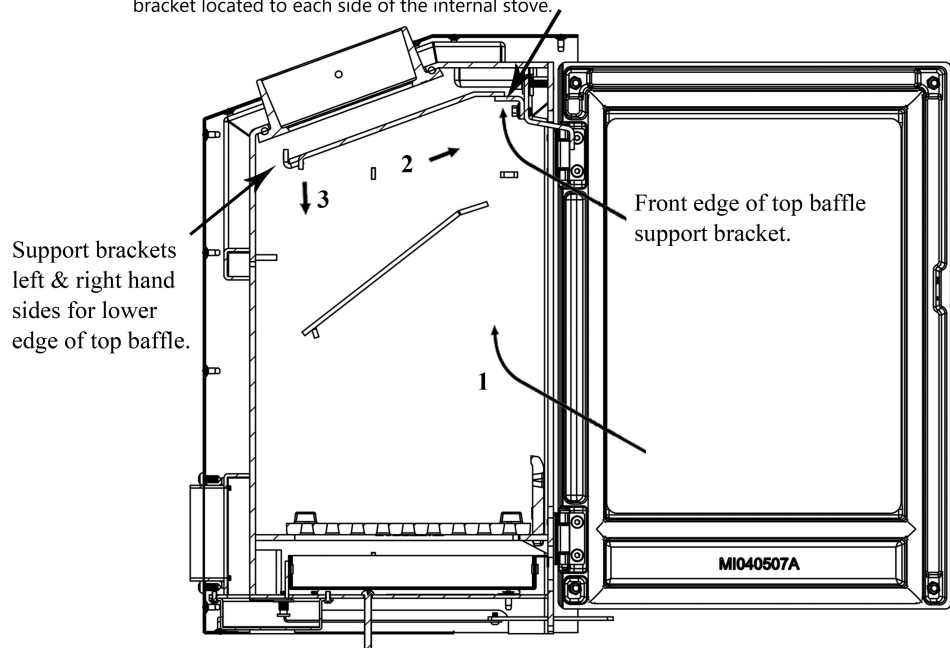
Fig 1.2 Top (lower) vermiculite baffle positioning.
