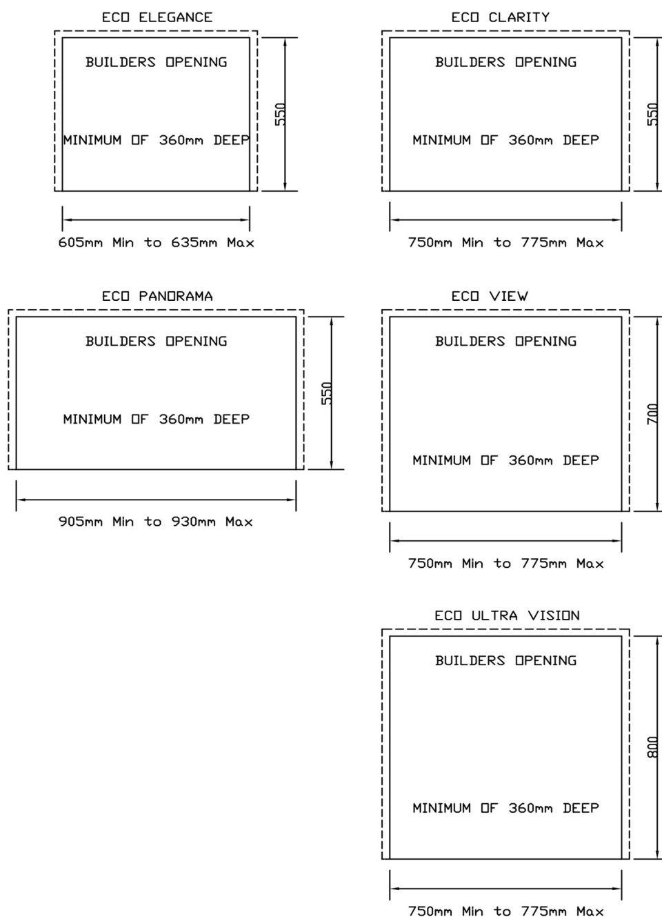
CHIMNEY BUILDERS OPENING DIMENSIONS.
